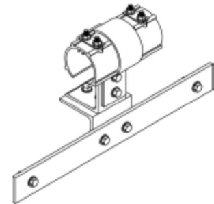
Assembled Unit
